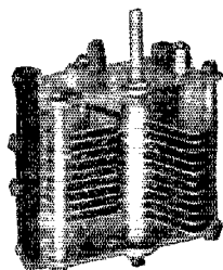
Transmitting type 164-B Capacity—.00022 mmfd.
