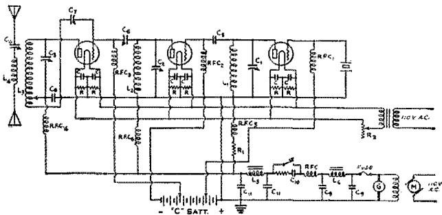
FIG. 1. — DIAGRAM OF THE TRANSMITTER AND POWER SUPPLY AT W9CJC
