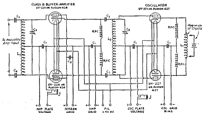
FIG. 1.—THE OSCILLATOR AND BUFFER-AMPLIFIER CIRCUIT
